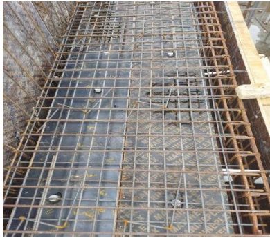
Roof terrace slab Reinforcement
